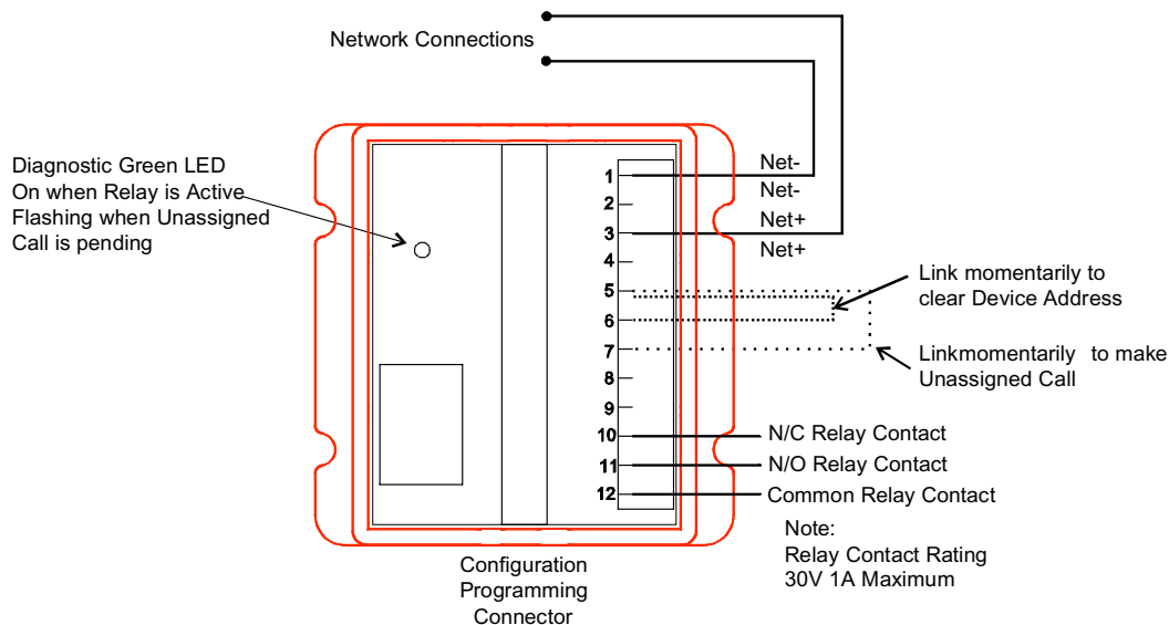
FIGURE 1 : Typical wiring scenario for the QT612 relay output device
